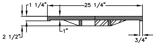
SECTION VIEW
