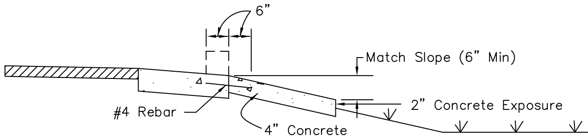
SECTION B-B
